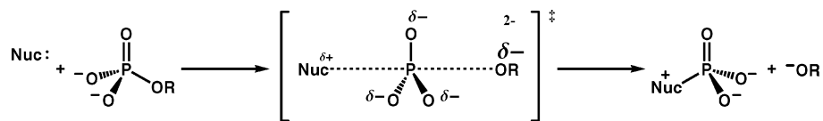
Scheme 2. Phosphate Monoester Hydrolysis through a Loose Transition State
