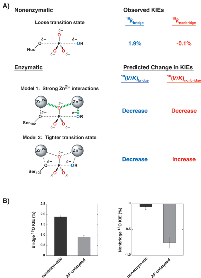
Figure 3. KIEs for AP-catalyzed reactions are different from the corresponding solution reaction. (A) Predicted direction of changes in KIEs relative to the solution reaction for two different models for behavior of phosphate monoester substrates in the AP active site. In model 1, the transition state is loose, similar to that in solution, and strong interactions with active-site metal ions lead to decreases in both ^{18}(V/K)_{\text{bridge}} and ^{18}(V/K)_{\text{nonbridge}} . In model 2, AP catalyzes phosphate monoester hydrolysis through a tighter transition state than that in solution. This model predicts a decrease in ^{18}(V/K)_{\text{bridge}} and an increase in ^{18}(V/K)_{\text{nonbridge}} based on comparisons to corresponding solution reactions. 16 (B) The observed values of both ^{18}(V/K)_{\text{bridge}} and ^{18}(V/K)_{\text{nonbridge}} for AP-catalyzed pNPP 2- hydrolysis decrease relative to the corresponding solution reaction, consistent with model 2. Isotope effects are expressed as a percentage difference from unity [KIE% = (KIE obs - 1) × 100]. Values for the nonenzymatic reaction are shown in black, and values for the AP-catalyzed reaction are shown in gray.
