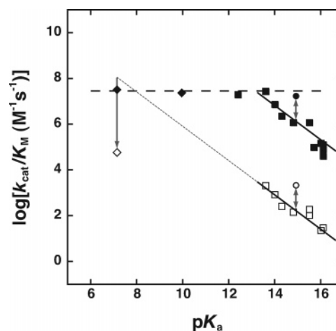
Figure 2. Compilation of kinetic data for the reactions of wt and R166S AP, represented by closed and open symbols, respectively. Reactions of alkyl phosphates (■, □) give values of \beta_{\text{lg}} of -0.85 \pm 0.1 and -0.66 \pm 0.1 respectively for reactions with wt and R166S AP. 10,12 Reactions of aryl phosphates (◆) with wt AP are limited by a nonchemical step (dashed line). 12 The rate constant for the reaction of the aryl phosphate pNPP 2- with R166S AP 22 deviates negatively from the value expected by extrapolation from the line for alkyl phosphates (dotted line and single-headed arrow). Rate constants for the reactions of mNBP 2- with wt and R166S AP (●, ○) deviate positively from the values expected from the line for alkyl phosphates (double-headed arrows).
