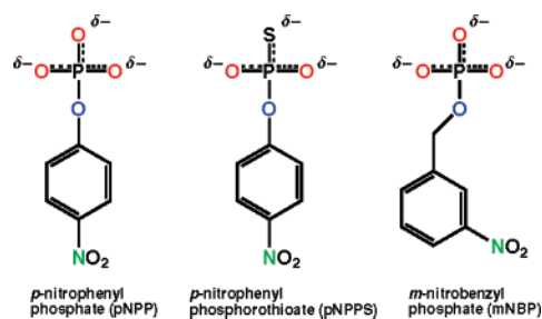
Figure 1. Phosphate and phosphorothioate esters for which isotope effects are reported: red, nonbridge phosphoryl oxygen atoms [ ^{18}(V/K)_{\text{nonbridge}} ]; blue, bridge oxygen atom, site of bond fission [ ^{18}(V/K)_{\text{bridge}} ]; green, nitrogen atom of the leaving group [ ^{15}(V/K) ]. The structures are depicted with partial double bonds to emphasize that the nonbridging oxygen atoms that contribute to ^{18}(V/K)_{\text{nonbridge}} are formally equivalent when the substrates are free in solution. For simplicity, the P–S and P–O bonds of pNPPS are depicted with the same partial double-bond character, although it is likely that the P–S bond has more single-bond character than the P–O bonds. 43,83
