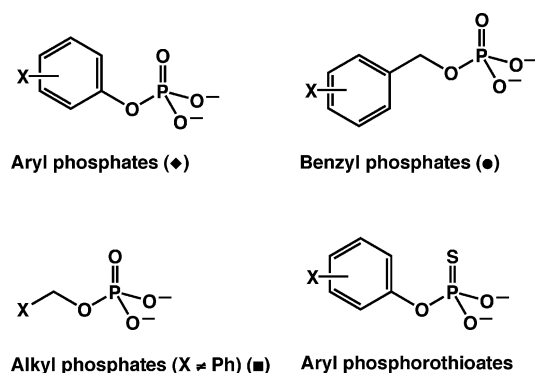
Figure 1. Phosphate and phosphorothioate esters for which isotope effects are reported: red, nonbridge phosphoryl oxygen atoms [ ^{18}(V/K)_{\text{nonbridge}} ]; blue, bridge oxygen atom, site of bond fission [ ^{18}(V/K)_{\text{bridge}} ]; green, nitrogen atom of the leaving group [ ^{15}(V/K) ]. The structures are depicted with partial double bonds to emphasize that the nonbridging oxygen atoms that contribute to ^{18}(V/K)_{\text{nonbridge}} are formally equivalent when the substrates are free in solution. For simplicity, the P–S and P–O bonds of pNPPS are depicted with the same partial double-bond character, although it is likely that the P–S bond has more single-bond character than the P–O bonds. 43,83
